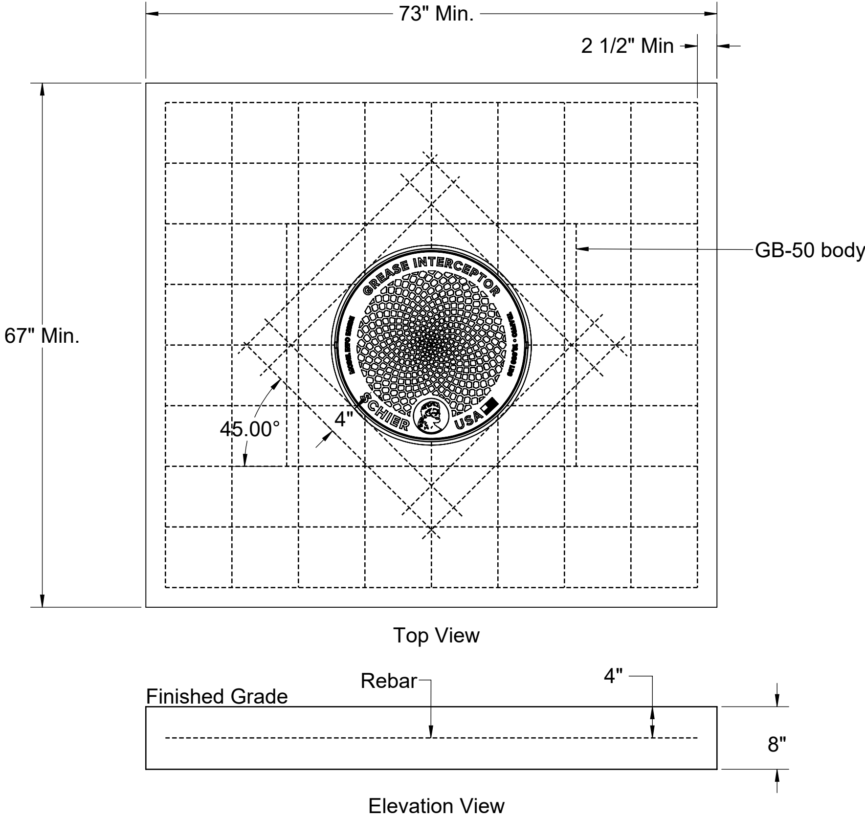
Concrete Slab Detail for H20/HS20 Loading
